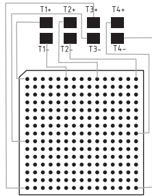
PBGA 225 PITCH 1,5MM
