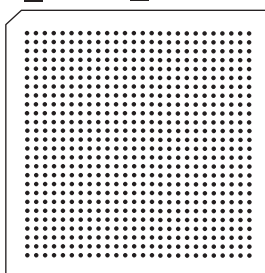
PBGA 676 PITCH 1,27MM
