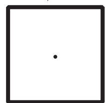
PLCC 68 PITCH 1,27MM
